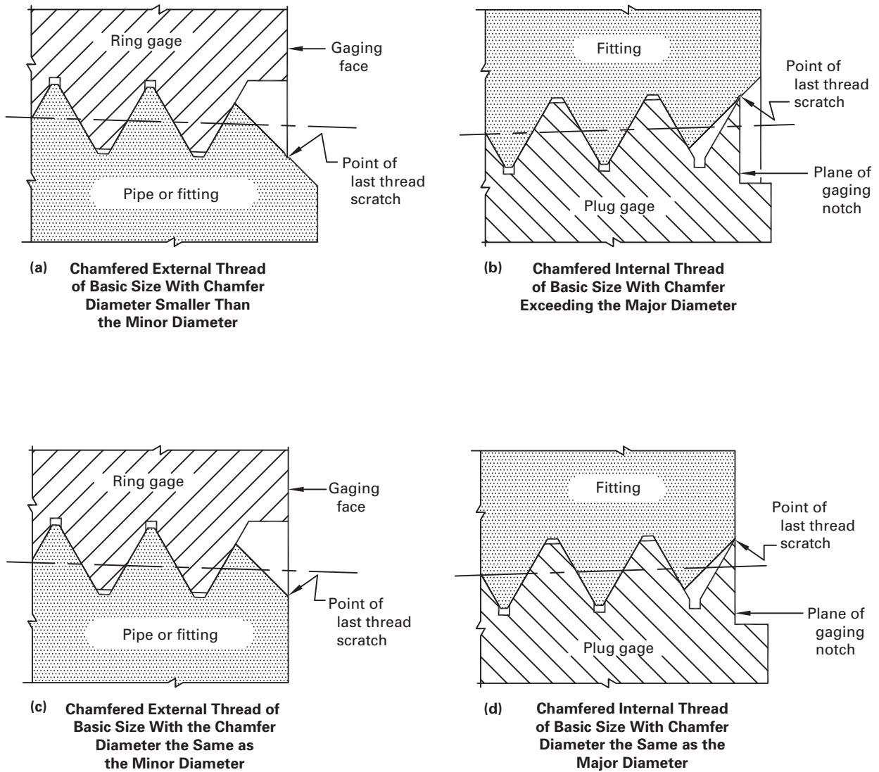
Fig. 5 Gaging of Chamfered Threads
