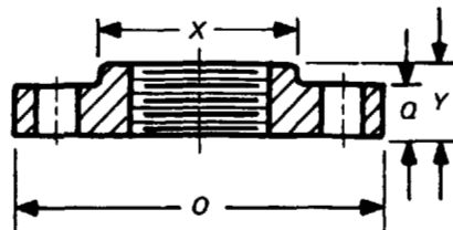
FIG. 2 CLASS 25 FLANGE
