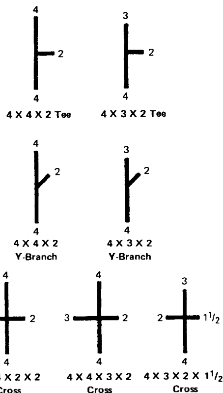
FIG. 1 IDENTIFICATION OF REDUCING FITTINGS
