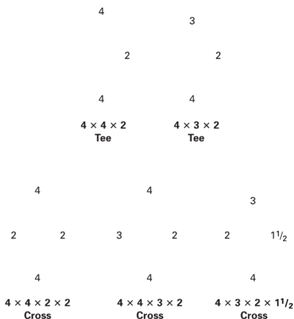
Fig. 1 Identification of Reducing Fittings
