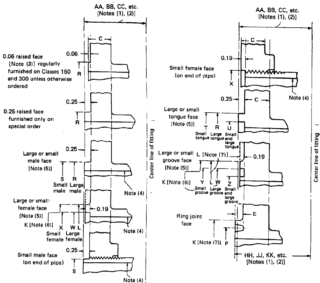
FIG. 7 END FLANGE FACINGS AND THEIR RELATIONSHIP TO FLANGE THICKNESS AND CENTER-TO-END AND END-TO-END DIMENSIONS 1,3
