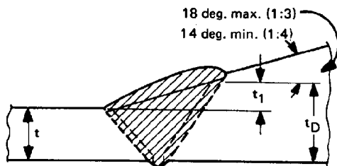
FIG. 12 BEVEL FOR OUTSIDE THICKNESS 1-4
