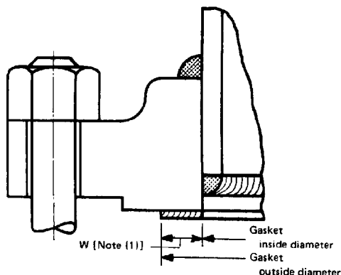
FIG. E8 3 SMALL TONGUE WIDTH GASKET WITH GASKET I.D. EQUAL TO PIPE O.D.
