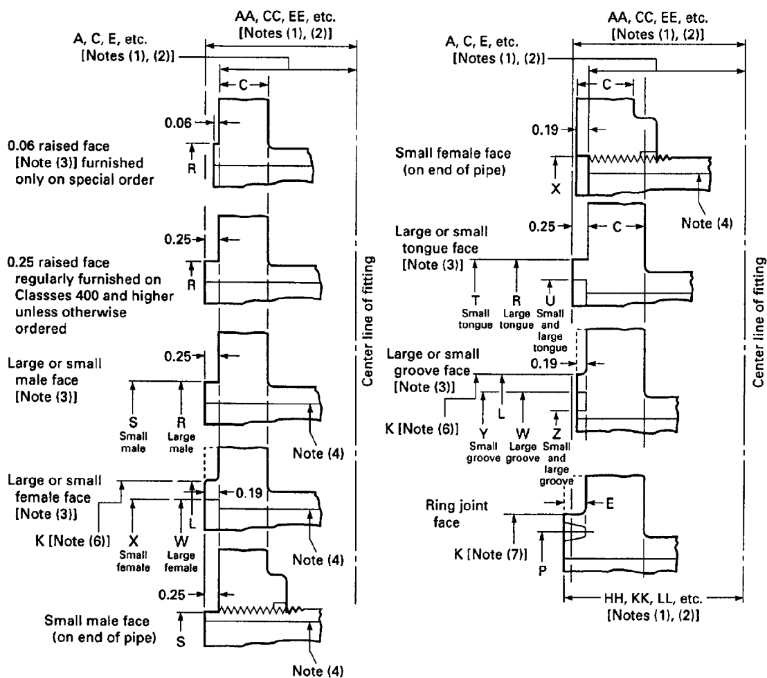
(a) FIG. 7 END FLANGE FACINGS AND THEIR RELATIONSHIP TO FLANGE THICKNESS AND CENTER-TO-END AND END-TO-END DIMENSIONS 1,3 (CONT'D)
