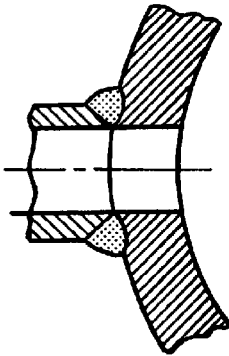
FIG. 5 BUTT WELDING FOR CONNECTIONS 1
