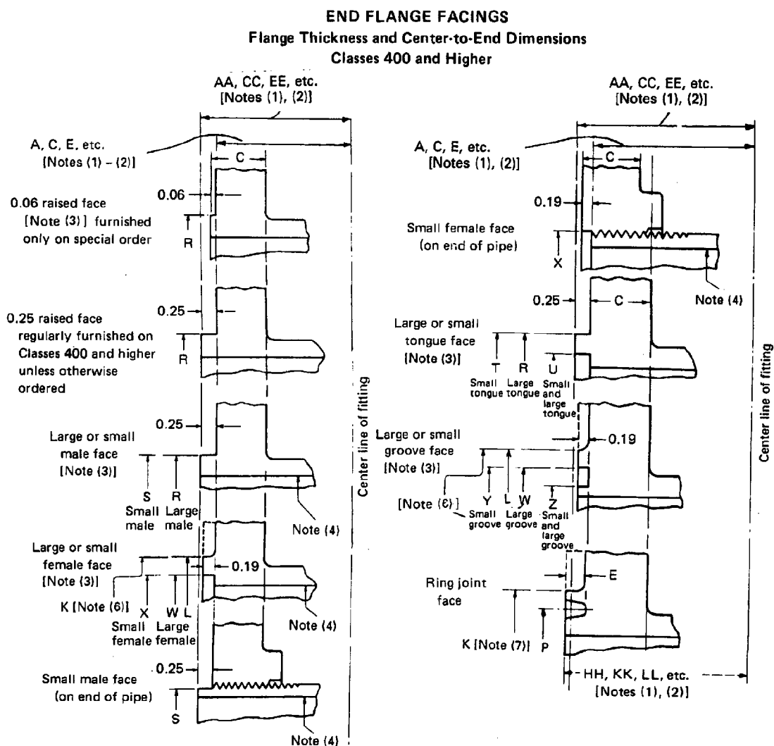
FIG. 7 END FLANGE FACINGS AND THEIR RELATIONSHIP TO FLANGE THICKNESS AND CENTER-TO-END AND END-TO-END DIMENSIONS 1,3 (CONT'D)
