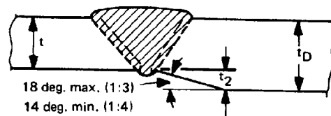
FIG. 13 BEVEL FOR INSIDE THICKNESS 1-3
