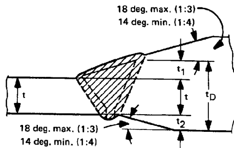
FIG. 14 BEVEL FOR COMBINED THICKNESS 1-4
