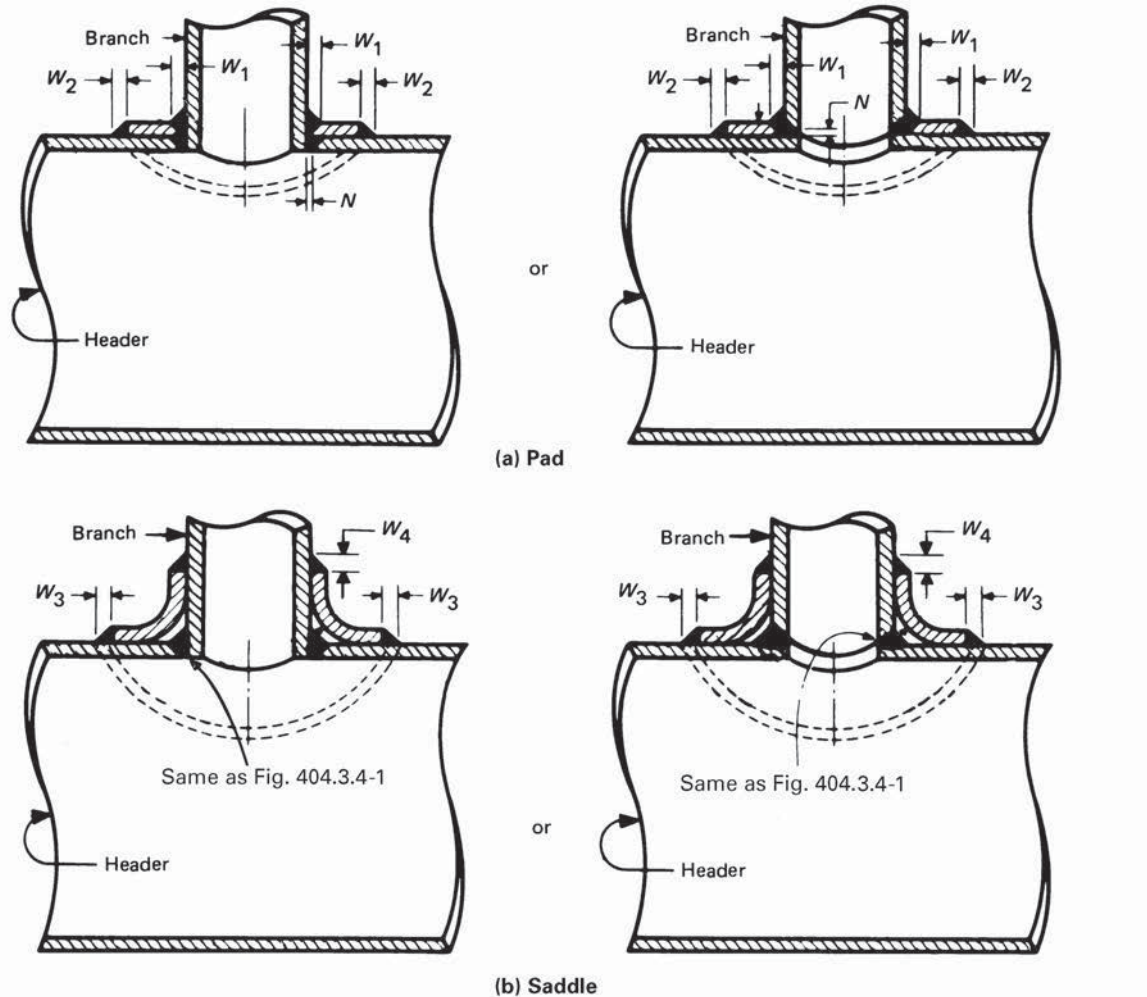
Fig. 404.3.4-2 Welding Details for Openings With Localized Type Reinforcement
