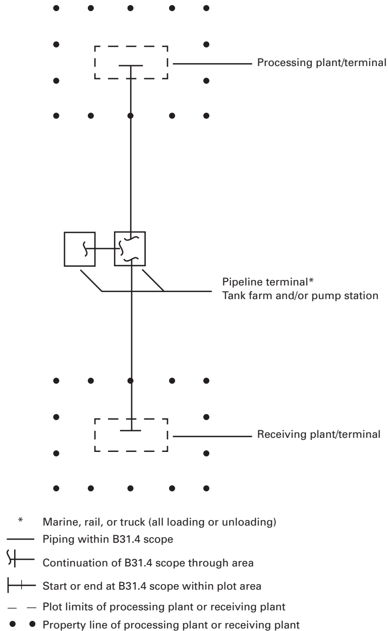
Fig. 400.1.1-3 Diagram Showing Scope of ASME B31.4 for Slurry Pipeline Systems
