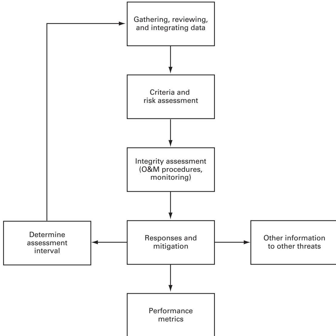
Fig. A-9.1-1 Integrity Management Plan, Weather-Related and Outside Force Threat (Earth Movement, Heavy Rains or Floods, Cold Weather, Lightning; Simplified Process: Prescriptive)
