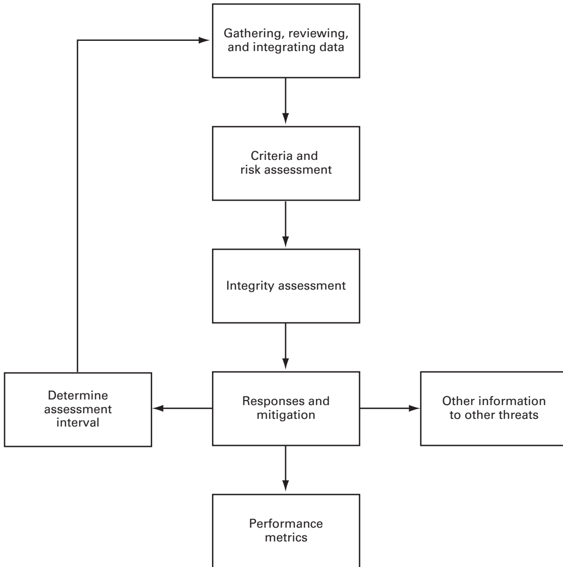
Fig. A-5.1-1 Integrity Management Plan, Construction Threat (Pipe Girth Weld, Fabrication Weld, Wrinkle Bend or Buckle, Stripped Threads/Broken Pipe/Coupling; Simplified Process: Prescriptive)
