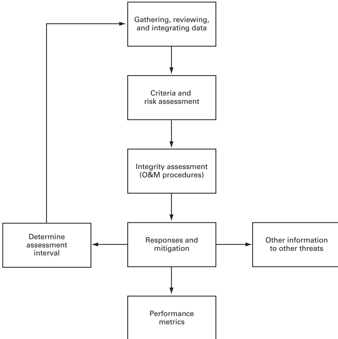
Fig. A-6.1-1 Integrity Management Plan, Equipment Threat (Gasket and O-Ring, Control/Relief, Seal/Pump Packing; Simplified Process: Prescriptive)
