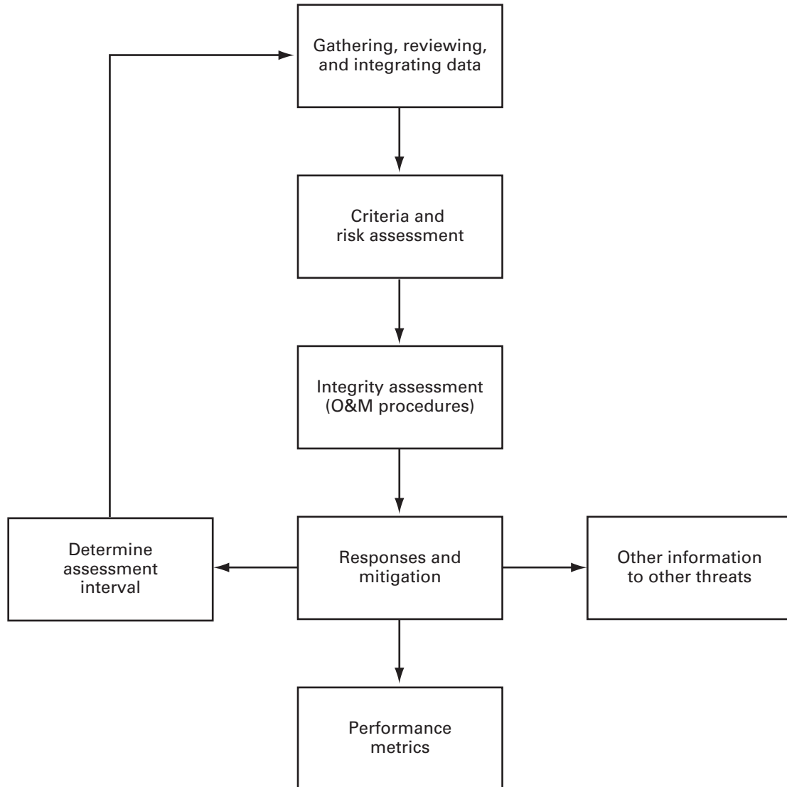
Fig. A-7.1-1 Integrity Management Plan, Third-Party Damage Threat [Third-Party Inflicted Damage (Immediate), Vandalism, Previously Damaged Pipe; Simplified Process: Prescriptive]
