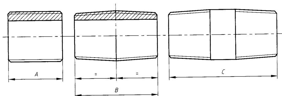
Running nipple (parallel thread)
