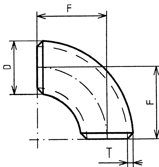
Figure 2 — 90° Elbow
