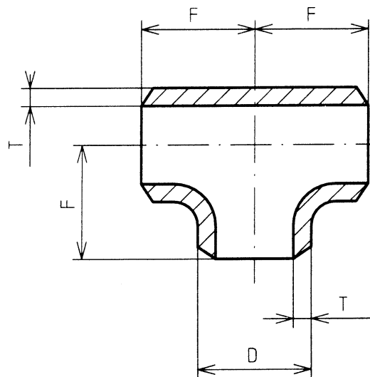
Figure 7 — Equal tee
