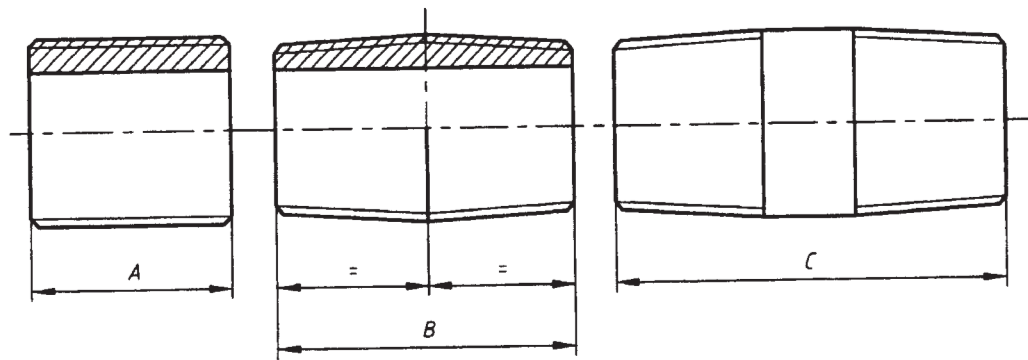
Running nipple (parallel thread)
