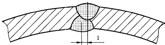
d) SAW 钢管焊缝焊偏
