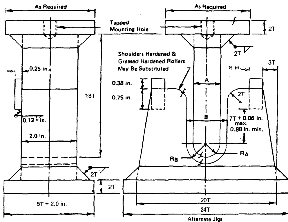
Guided-Bend Test Jig Dimensions
