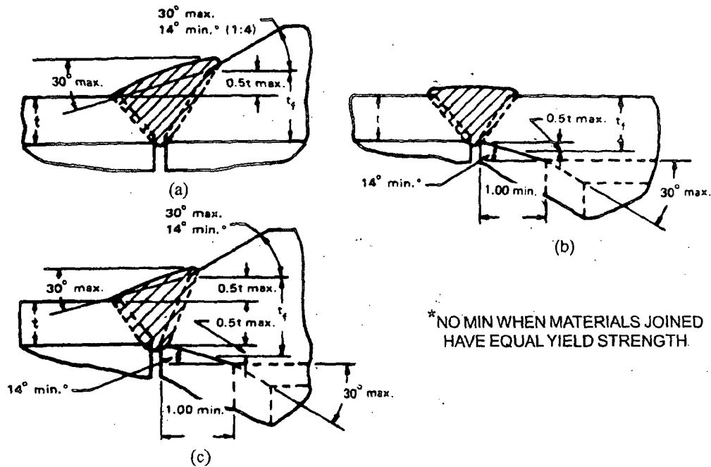
ACCEPTABLE DESIGN FOR UNEQUAL WALL THICKNESS (See Section 8.1.1)
