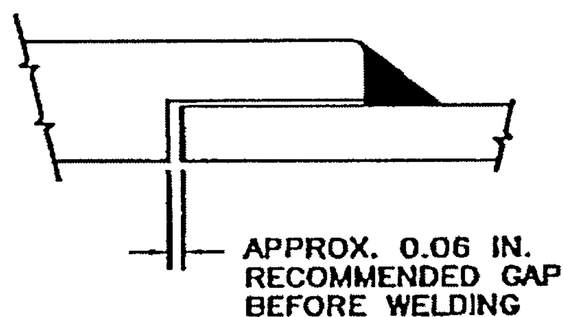
Figure 1 - Welding Gap
