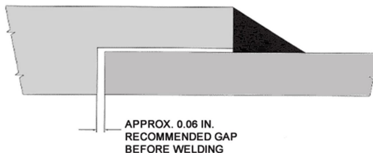
Figure 1 – Welding Gap
